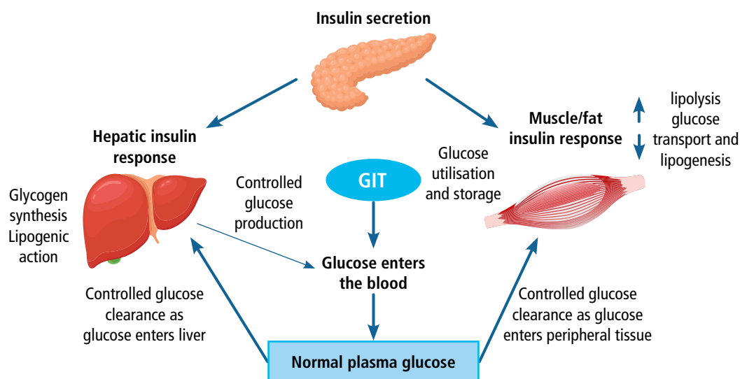
Figure 1. Normal regulation of plasma glucose
